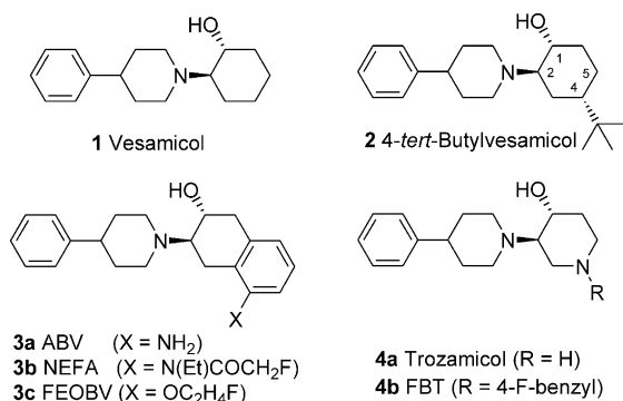
Figure 1. Ligands for the vesicular acetylcholine transporter (VACHT).
