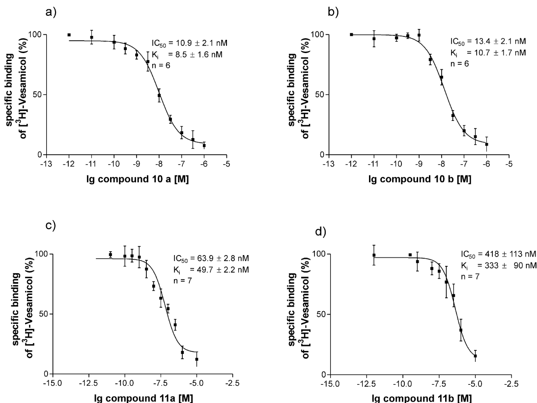
Figure 2. Concentration-dependent displacement of [ 3 H]vesamicol binding in rat brain membranes by 4- O -benzylether 10a (a) and 10b (b) and 5- O -benzylether 11a (c) and 11b (d). Using nonlinear regression analysis data were best fitted to a one-site-binding model in all cases.
