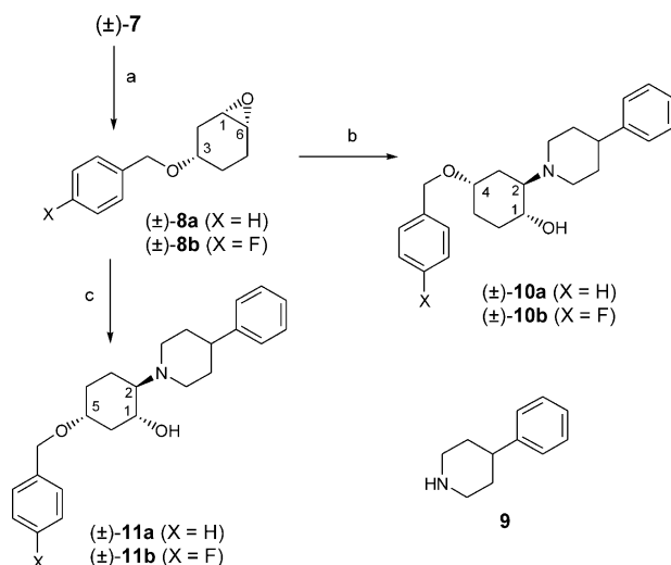
Scheme 2. Synthesis of 4-substituted (10) and 5-substituted vesamicol analogues (11). Reagents and conditions: (a) NaH/DMF, benzyl bromide or 4-fluorobenzyl bromide (8a, 73%; 8b, 61%); (b) 9, EtOH, 55–60°C, 3 d (10a, 73%; 10b, 59%); (c) 9, MeCN, LiClO 4 , 20°C, 16 h (11a, 89%; 11b, 86%).
